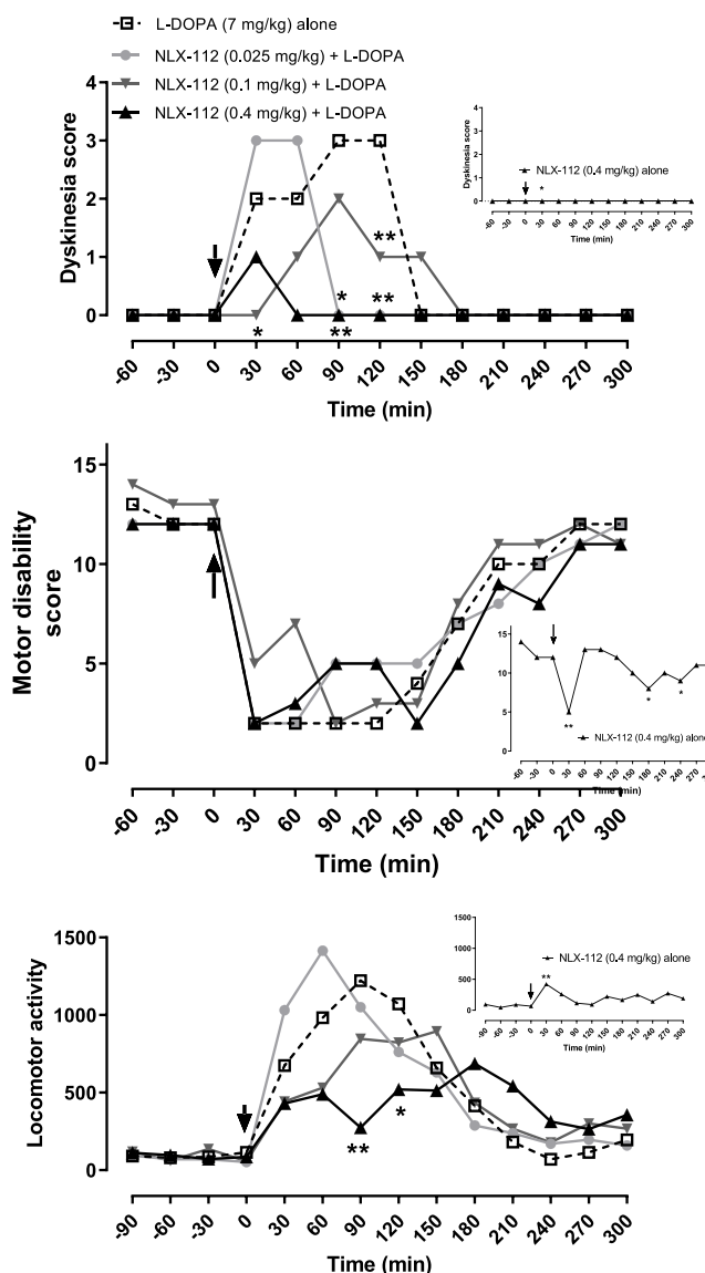
Fig. 2. Time course of effects of NLX-112 in combination with L-DOPA (main panels) or alone (insets). Main panels: NLX-112 or vehicle and L-DOPA (7 mg/kg) were administered p.o. at t = 0 min (arrows). Benserazide was administered at t = -60 min. For dyskinesia and motor disability, data are presented as median values and were analyzed by two-way ANOVA on transformed data [ y = \sqrt{\text{y}} ]. For locomotor activity, data are presented as mean values, and were analyzed by two-way ANOVA on raw data. * p < 0.05 , ** p < 0.01 , versus L-DOPA alone at the considered time point, Dunnett's post-hoc tests. N = 7 per group. Insets: NLX-112 was administered alone p.o. at t = 0 min (arrows). For dyskinesia and motor disability, data are presented as median values and were analyzed by one-way ANOVA on transformed data [ y = \sqrt{\text{y}} ]. For locomotor activity, data are presented as mean values, and were analyzed by one-way ANOVA on raw data. * p < 0.05 , ** p < 0.01 versus value at t = -60 min (dyskinesia and motor disability) or t = -90 min (locomotor activity), Dunnett's post-hoc tests.
