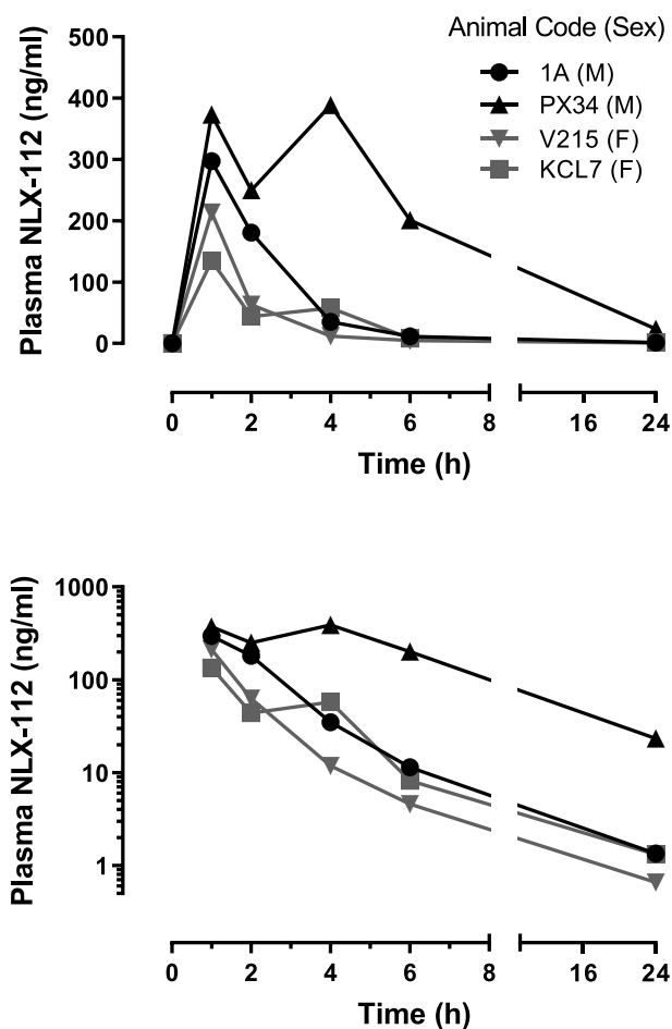
Fig. 1. Plasma Levels of NLX-112 in Marmosets. Symbols represent the mean of duplicate measures taken from the same plasma sample following administration of 0.4 mg/kg p.o. NLX-112 was quantified by LC-MS/MS. The same data are plotted on a linear scale y-axis (upper panel) and on a log 10 scale y-axis (lower panel). M: male, F: female.
