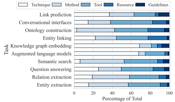
Figure 6: Percentage of contribution type by tasks.
