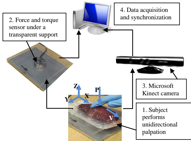
Fig. 4. Schematic arrangement of an experimental setup: The subject is performing palpation with one finger (1) – the main palpation features: applied pressure P , velocity V and trajectory in three-dimensional space XYZ ; the applied force is measured using a force/torque sensor, mounted under the transparent support plate (2) and the trajectory is measured by a three-dimensional vision system (3). All acquired sensor data is synchronized and processed
