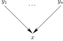
FIGURE 1. Basic attack formation in an argumentation network.
