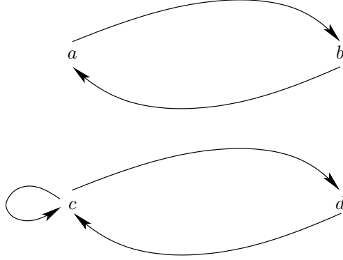
FIGURE 13. Augmented network of Figure 2 with node a as c and b as d and an extra cycle.
