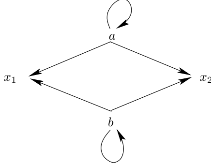
FIGURE 8. Mirrored network of Figure 7.
