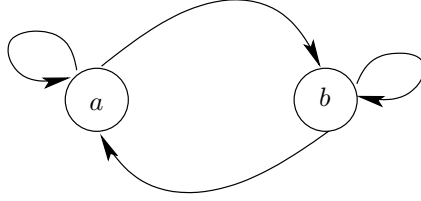
FIGURE 6. Network for Example 3.5.
