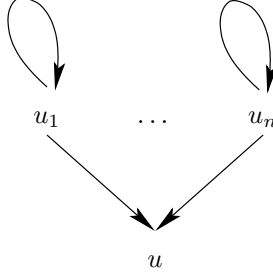
FIGURE 9. Multiple attacks by undecided nodes.
