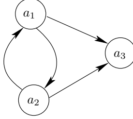
FIGURE 5. Figure 2 of “A probabilistic semantics for abstract argumentation” [13].
