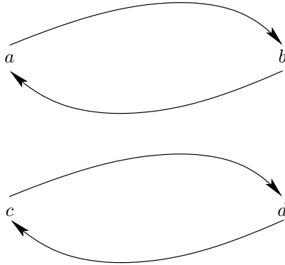
FIGURE 11. A network with two cycles.
