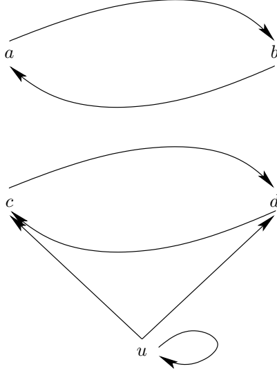
FIGURE 12. A self-attacking node attacking one of the cycles in the network of Figure 11.
