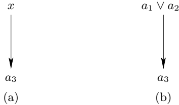
FIGURE 14. (a) A network and (b) one of its instantiations with x = a_1 \vee a_2
