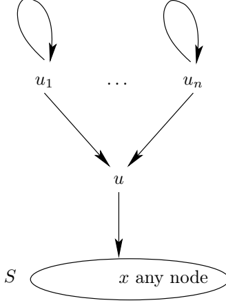
FIGURE 10. Scenario depicted in Remark 4.1.
