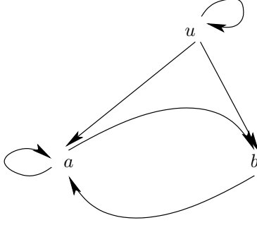
FIGURE 3. The network of Figure 2 with an extra undecided node u attacking all nodes.
