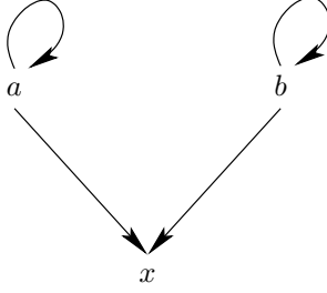
FIGURE 7. A network with Method 1 and Method 2 probabilities.
