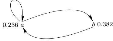
FIGURE 15. The \text{Eq}_{\text{inv}} solution to the networks of Figures 2 and 3
