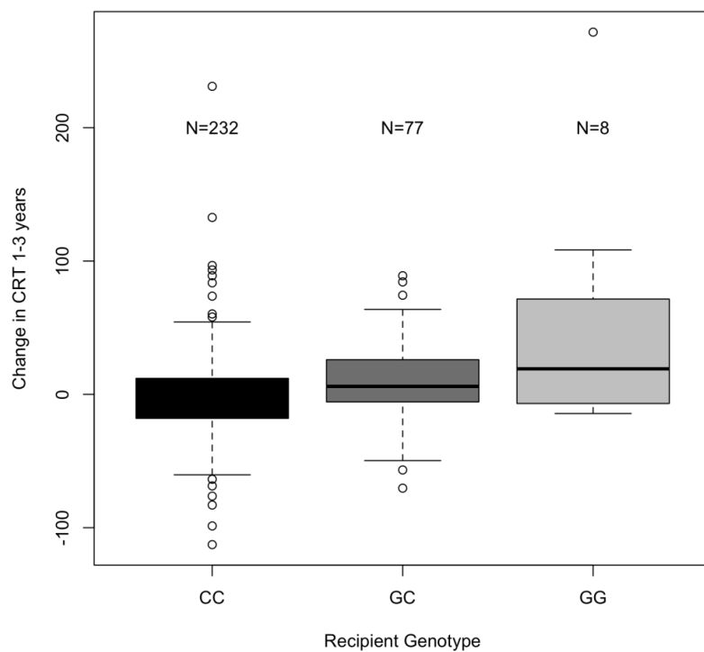
Figure 2. Box plots of KCL 1- vs 3-year serum creatinine stratified by recipient rs930507 genotype. Numbers in each group are also indicated.
