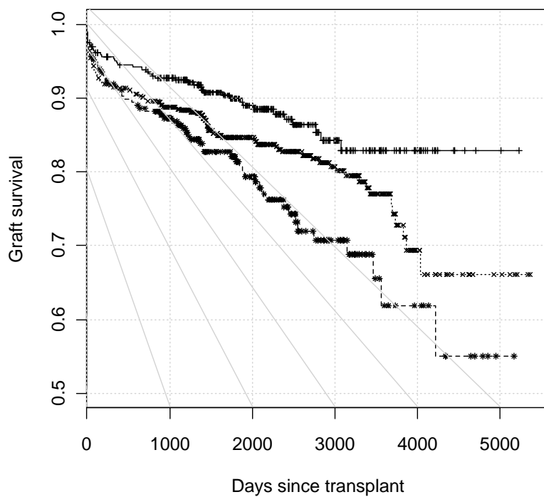
Figure 1. Kaplan-Meier plots of graft survival stratified by donor rs4935047 genotype. Top line (solid, straight ticks) is for the major homozygote; middle line (dotted, cross ticks) is for the heterozygote; bottom line (dashed, star ticks) is for the minor homozygote.
