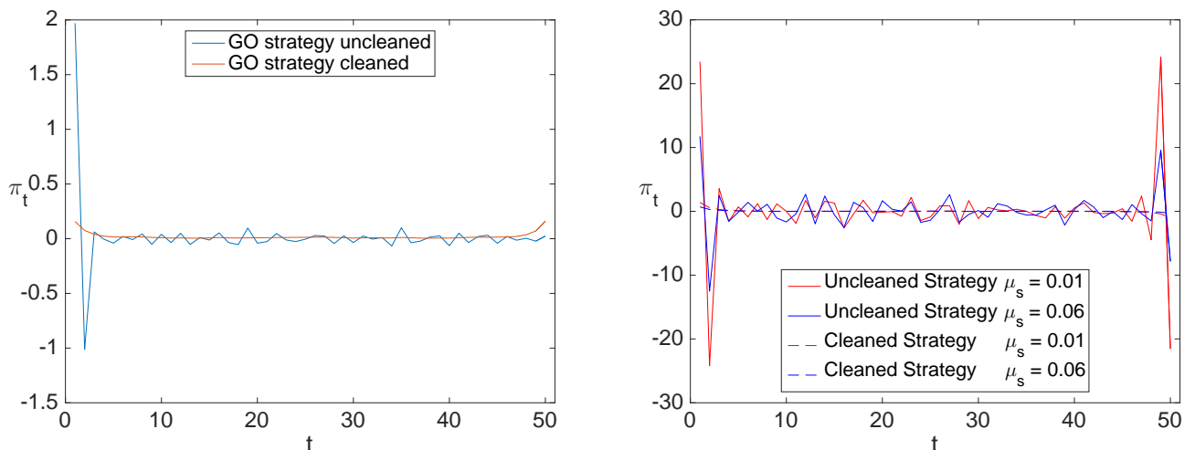
FIG. 8: Left: globally optimal strategy for the S&P500, showing both results before and after cleaning. Right: optimal strategies for the two target returns of \mu_S = 0.01 and 0.06 indicated in Fig. 7 above.
