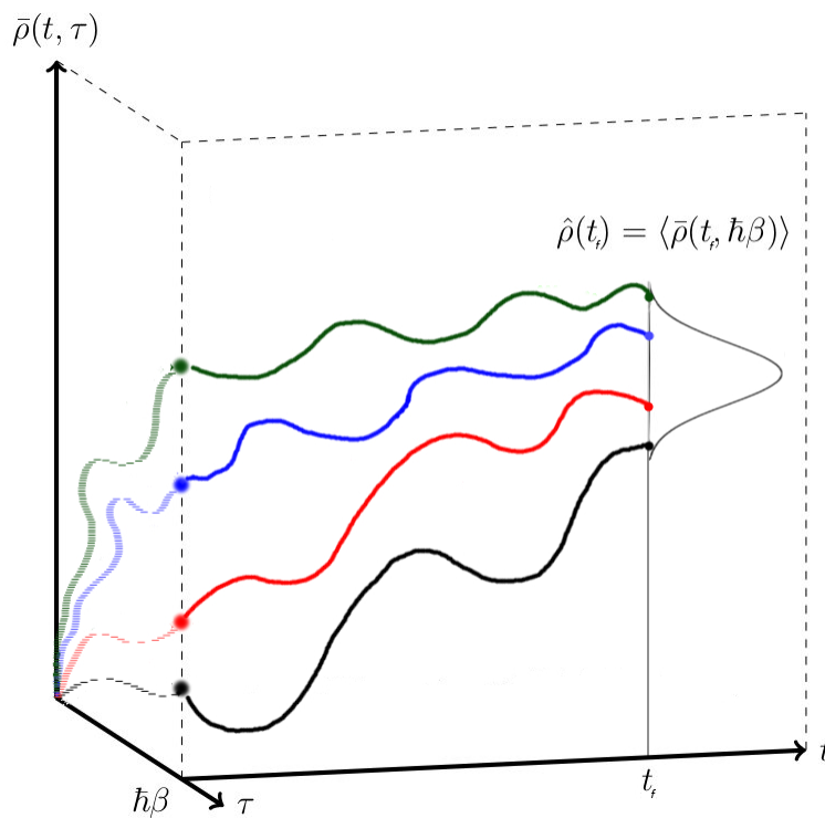
Figure 2. Representative trajectories for the evolution of the system. First there is an evolution in imaginary time up to \tau = \beta\hbar , before evolving in real time from this point up to time t_f . Different colours correspond to different simulations associated with particular manifestations of the noises. The average of the final points gives the physical density matrix at that time (indicated at time t_f ).
