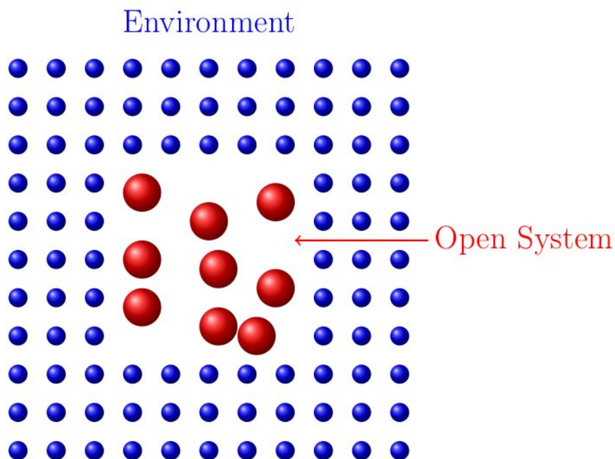
Figure 1. Schematic of the system. The Q system will be described by the q coordinates, and its environment, the X system, with \xi coordinates ( x in normal modes).
