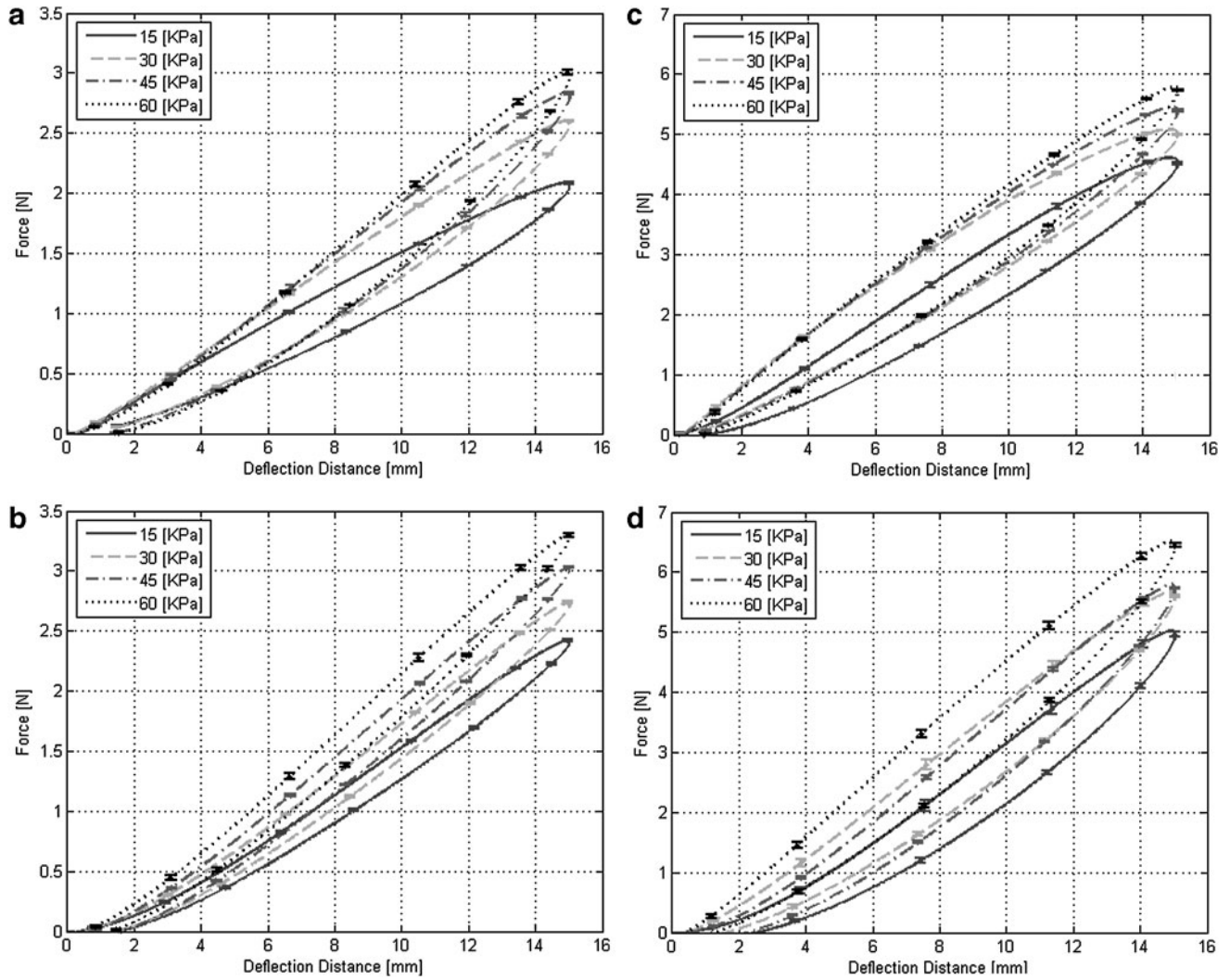
FIG. 4. Deflection distance versus force at the link tip laterally applied for samples (a), (b), (c), and (d) at 15, 30, 45, and 60 kPa. Standard deviation values ordered by increasing pressure level: (a) 0.007, 0.006, 0.0144, 0.009; (b) 0.009, 0.008, 0.008, 0.018; (c) 0.018, 0.016, 0.013, 0.016; (d) 0.041, 0.039, 0.017, 0.036.
