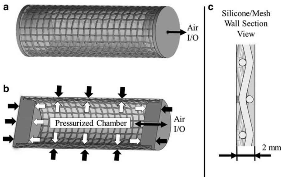
FIG. 1. CAD drawings of the stiffness-controllable link: overview of the link assembly (a), longitudinal section view of the link (b) showing the I/O channel for pressurized air, with white arrows showing the force distribution of the pressurized air inside the internal chamber and single-headed black arrows the force distribution of the reaction forces of the link. (c) Subfigure shows a longitudinal magnified section of the wall link, showing the mesh embedded in a 2 mm silicone layer.
