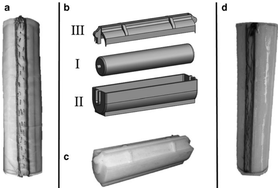
FIG. 2. Fabrication stages of the link: mesh sewn in the shape of a cylinder (a), mold components [I, II, and III (b)], and mold assembled (c). (d) Shows the link after demolding and removing of the silicone excess.
