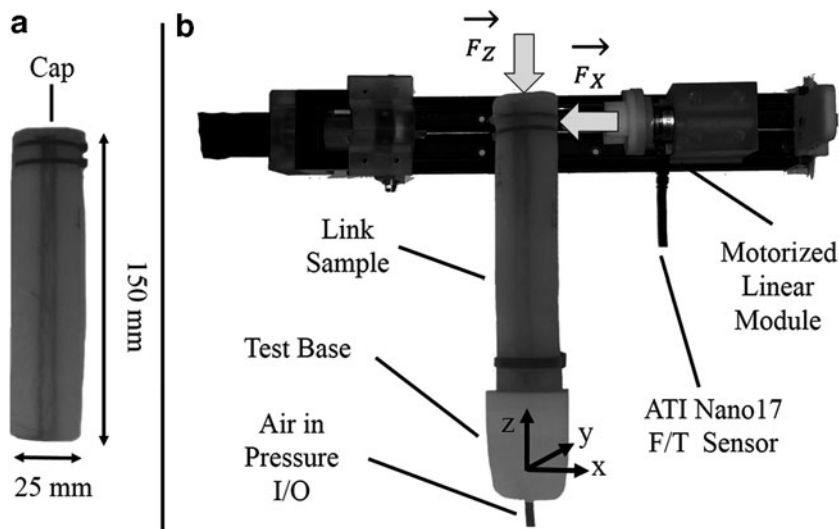
FIG. 3. Link sample with 3D printed cap embedded for stiffness test (a) and setup for the lateral stiffness tests at the tip (b) direction of the lateral force F_x and of the longitudinal force F_z applied during the tests are marked.
