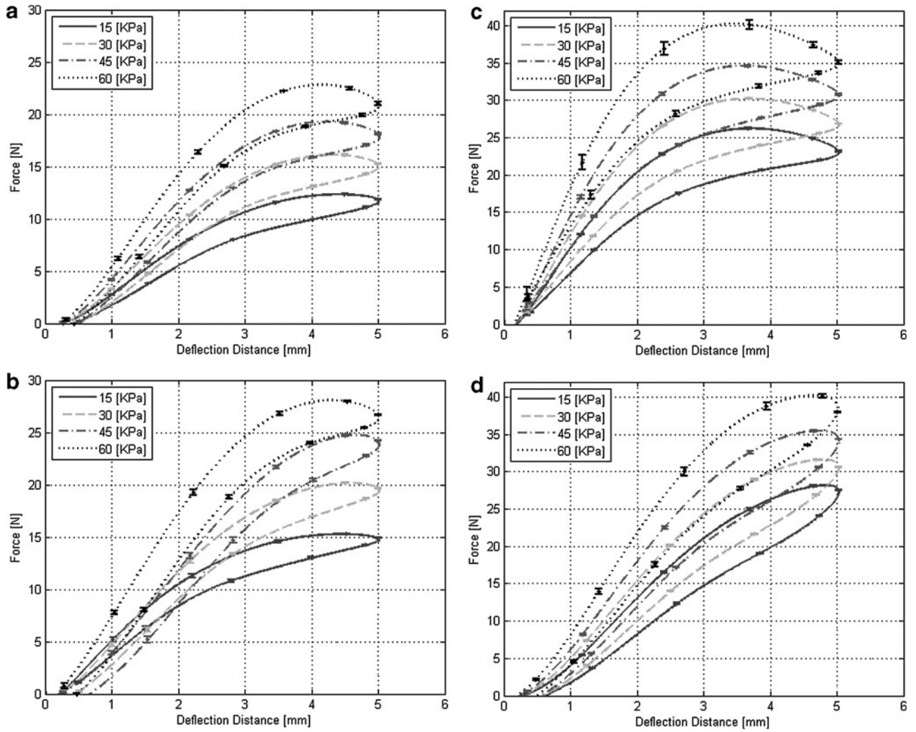
FIG. 5. Deflection versus force at the link tip longitudinally applied for samples (a), (b), (c), and (d) at 15, 30, 45, and 60 kPa. Standard deviation values ordered by increasing pressure level: (a) 0.051, 0.080, 0.089, 0.153; (b) 0.150, 0.136, 0.178, 0.179; (c) 0.133, 0.123, 0.206, 0.536; (d) 0.095, 0.100, 0.121, 0.255.
