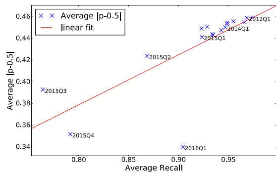
(c) SVM
