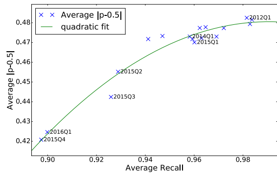
(a) XGBoost
