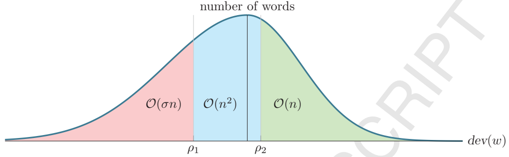
Figure 1: For a word x , the words for which E(w) > 0 are the ones of the form w = aub , where au and ub are factors of x and a, b \in \Sigma , not necessarily distinct. There are \mathcal{O}(n^2) such words (see Fact 1 in this regard). We have shown that the \rho_1 -avoided words are \mathcal{O}(\sigma n) [2]. In this article, we show that the \rho_2 -overabundant ones are \mathcal{O}(n) .
