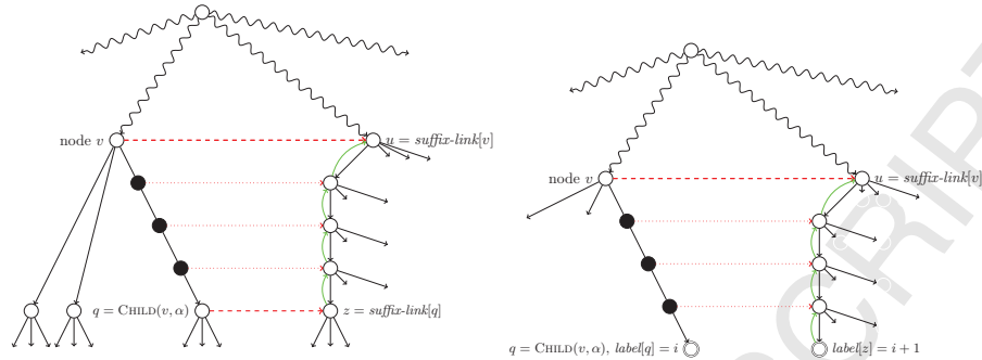
Figure 3: The above figures illustrate the nodes (implicit or explicit) considered in a step (lines 6-37) of Algorithm 1. The figure on the left presents the case where \text{CHILD}(v, \alpha) is an internal node, while the right one the case that it is a leaf. Black nodes represent implicit nodes along the edge (v, q) that we have to consider as potential w_p , and the red dotted line joins them with the respective (white) explicit node that represents the longest suffix of this w_p , i.e. w_i .
