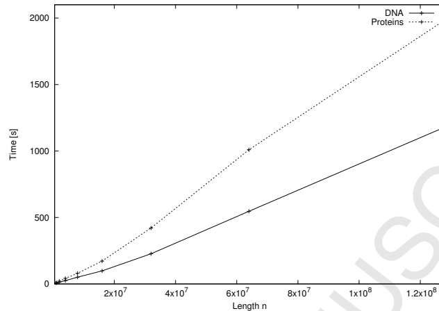
Figure 4: Elapsed time of Algorithm 1 using synthetic DNA ( \sigma = 4 ) and proteins ( \sigma = 20 ) sequences of length 1M to 128M.
