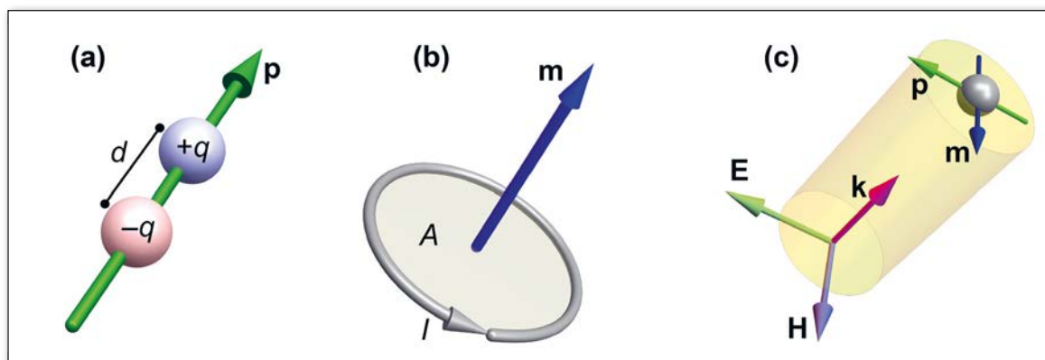
◀ FIG. 1: (a) The electric dipole moment vector \mathbf{p} is the product between the charge constituting each of its poles q , and their separation distance d . (b) The magnetic dipole moment vector \mathbf{m} is the product between the amplitude of a circulating current I and the area it encloses A\hat{n} , in a direction \hat{n} normal to the area. Both converge to point sources in the appropriate limit. (c) A polarizable particle being illuminated by an incident beam with wave-vector \mathbf{k} , electric field \mathbf{E} , and magnetic field \mathbf{H} . The particle becomes polarized and behaves like a dipolar source with dipole moments proportional to the incident fields \mathbf{p}=\alpha_e\mathbf{E} and \mathbf{m}=\alpha_m\mathbf{H} with \alpha_{e/m} representing complex proportionality constants, which are the particle's electric and magnetic polarizability.
