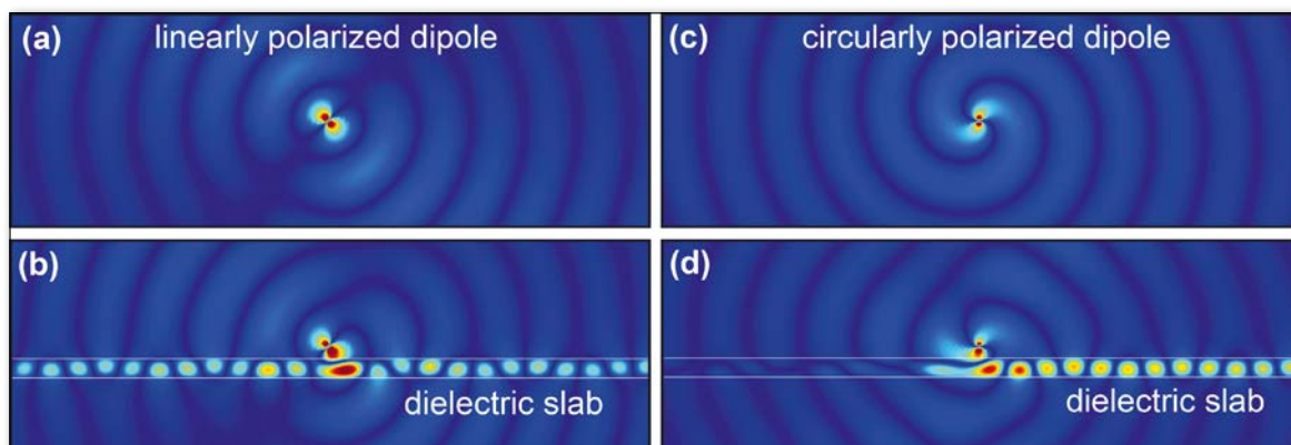
◀ FIG. 2: Snapshot of radiated magnetic field amplitude of a linearly (a,b) and circularly (c,d) polarized electric dipole radiating either in free-space (a,c) or at a subwavelength distance 0.1\lambda near a dielectric waveguide (b,d). The phenomenon exists for any kind of waveguide. In this figure we chose a dielectric slab with refractive index n=3 and thickness t=0.2\lambda .
