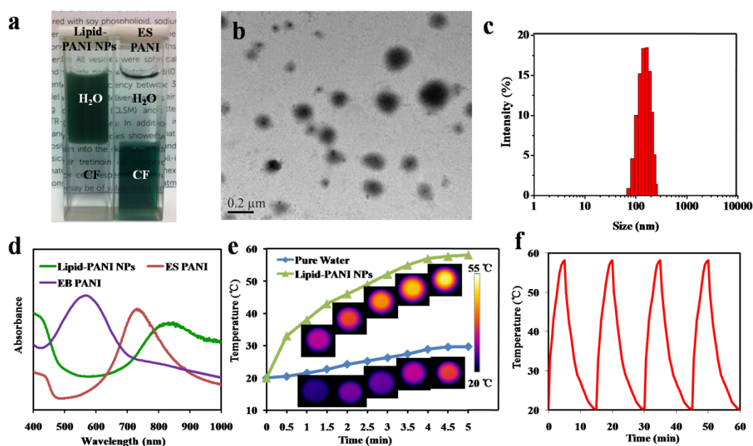
Figure 2. a) Solubility test of Lipid-PANI NPs (left) and ES PANI (right) in chloroform (lower phase) and water (upper phase). b) TEM image of Lipid-PANI NPs (scale bar = 0.2 μm). c) Size distribution of Lipid-PANI NPs. d) UV-Vis-NIR absorption spectra of Lipid-PANI NPs dispersed in water, ES PANI and EB PANI dissolved in chloroform. e) Temperature evolution curves and photothermal images of pure water and aqueous solution of Lipid-PANI NPs over a period of 5 min following exposure to the NIR laser (808 nm, 2 W cm -2 ). f) Temperature monitoring of a Lipid-PANI aqueous suspension at the concentration of 0.2 mg/mL during for successive cycles of an on-and-off laser.
