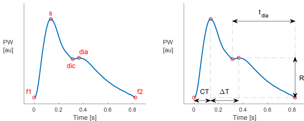
Figure 2. Extraction of features from photoplethysmogram (PPG) pulse waves (PWs), shown for the wrist PPG PW: (left) Fiducial points were identified; (right) Feature measurements were extracted from the positions of fiducial points. Exemplary features are shown; the full list is provided in [11].
