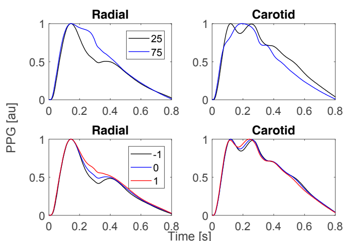
Figure 4. Photoplethysmogram (PPG) pulse waves (PWs) at the wrist (radial artery, left ) and neck (carotid artery, right ) sites, shown for subjects aged 25 and 75 ( upper panels) and for different levels of arterial stiffness ( lower panels). The lower plots show the PWs obtained when varying the arterial stiffness by \pm 1 standard deviation from typical values.
