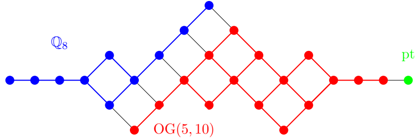
Figure 3: P_{\omega_6} -orbits in E_6/P_{\omega_1}
