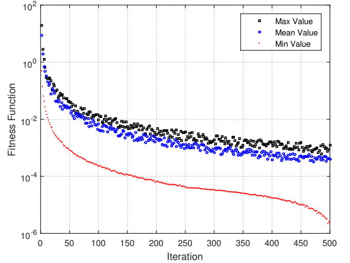
Fig. 2. Convergence of IWO for the KKT condition \partial \Upsilon / \partial \lambda_n^* = 0 .
