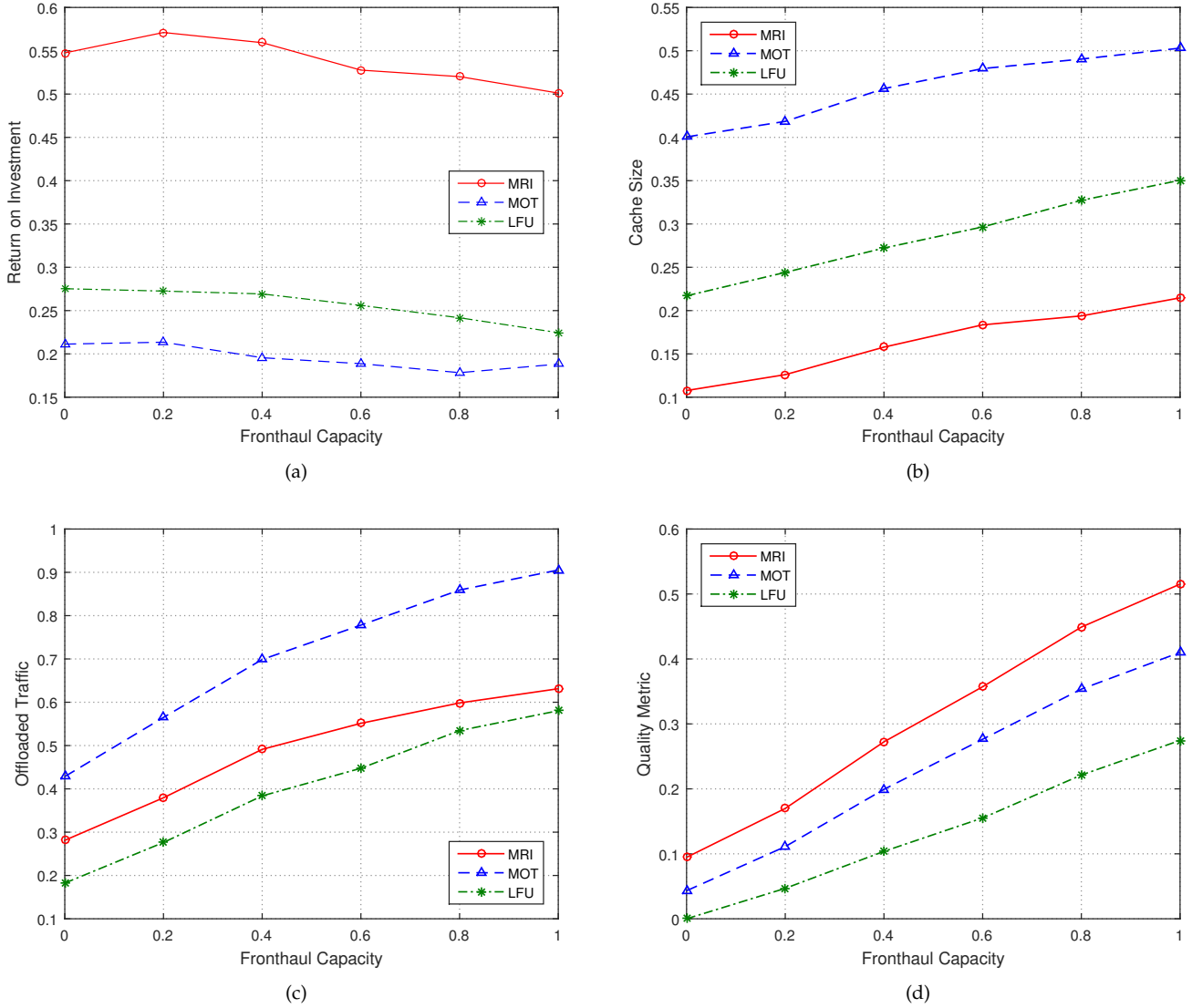
Fig. 4. Scenario 2 - varying fronthaul capacity: (a) return on investment; (b) cache size; (c) offloaded traffic; (d) quality metric.
