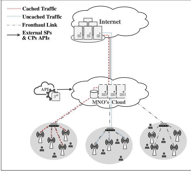
Fig. 1. Cloud-based virtual caching architecture.
