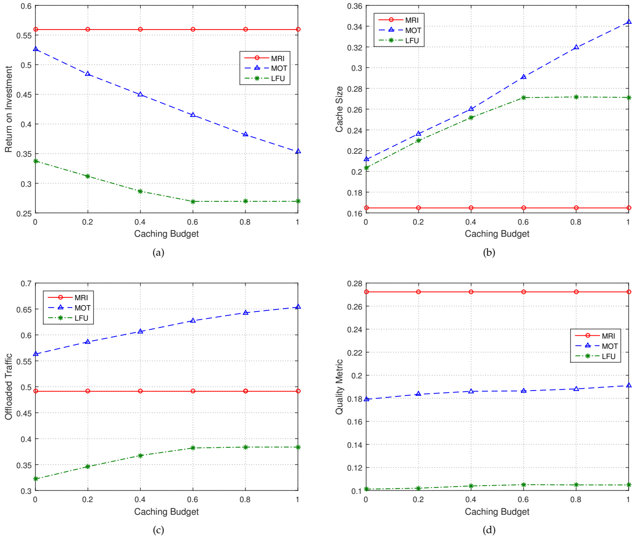
Fig. 5. Scenario 3 - varying caching budget: (a) return on investment; (b) cache size; (c) offloaded traffic; (d) quality metric.
