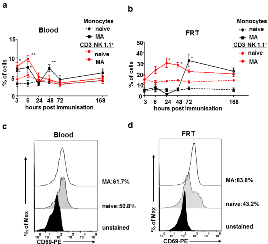
Figure 6. Skin immunisation promotes the early recruitment of ILC1 and monocytes to the FRT. (a,b) Frequency of ILC1 ( CD45^+NK1.1^+ CD3^- ) and monocytes ( CD45^+Ly6C^+CD11b^+MHCII^- ) in peripheral blood (a) and FRT tissue (b) at the indicated time points from naive or Ad-CN54 gag skin MA immunised mice for each time point (c,d). Representative flow cytometry profile of CD69 expressed on ILC1 isolated from peripheral blood (c) or FRT tissue (d), 24 h after Ad-CN54 gag immunisation or from naive controls. Data are from three independent experiments (n=3-10 per group). *p<0.05, **p<0.01 by one-way ANOVA, error bars show s.e.m.
