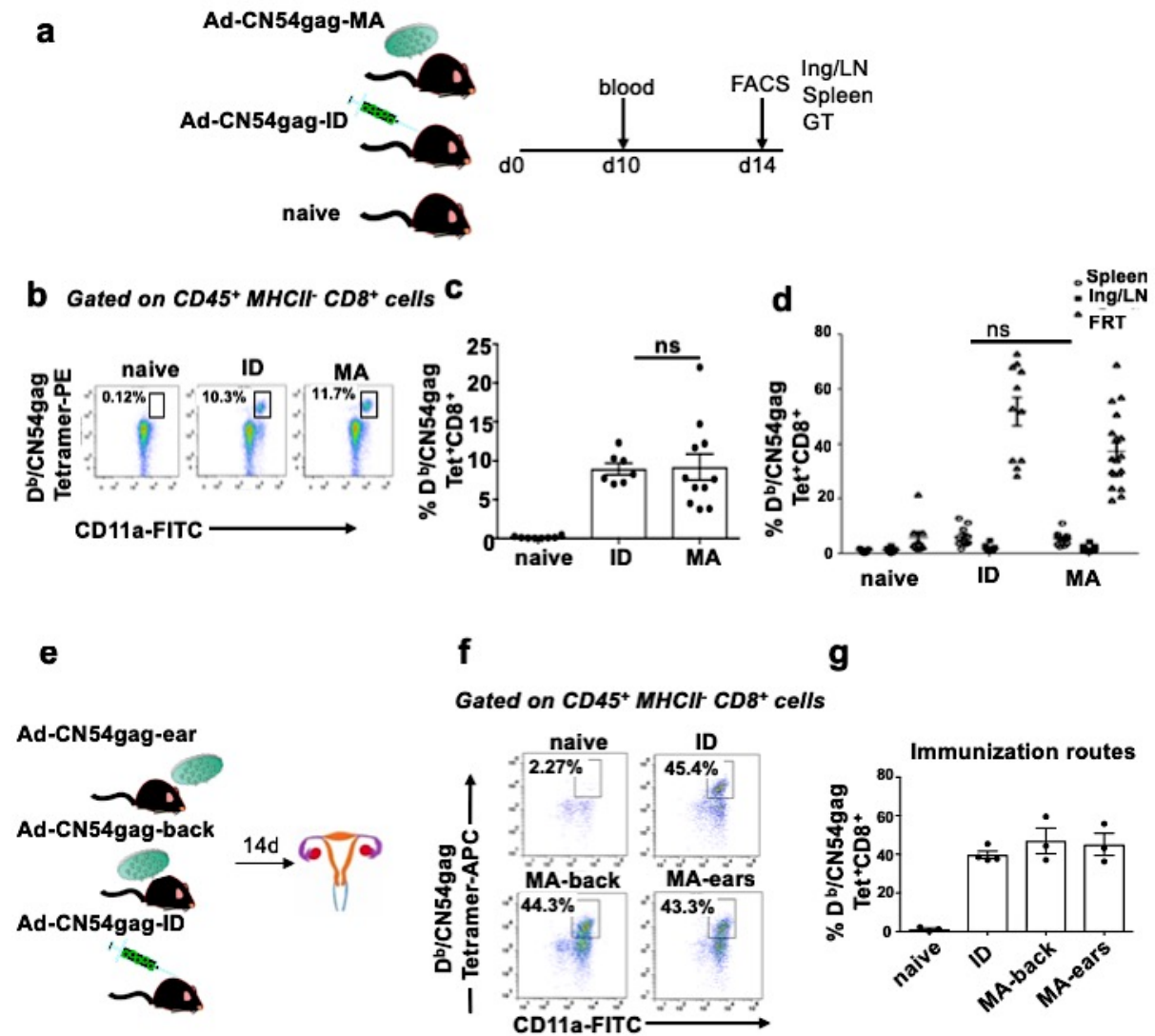
Figure 1. Skin immunisation irrespective of anatomic site recruits CD8^+ T cells to the FRT (a) Experimental design. (b, c, d) Flow cytometry plots and graphs showing frequencies of CD8^+ D^b/CN54gag tet ^+ cells in blood (day 10) and indicated tissues (spleen, inguinal LN and FRT) on day 14 after ID or MA (back skin) immunisation with Ad-CN54gag. Data are from four independent experiments ( n=7-18 mice per group). (e) Experimental design. Mice were immunised by MA either to the dorsal surface of the ear or to back skin or ID (f, g) Flow cytometry plots and graph showing frequencies of CD8^+ D^b/CN54gag tetramer ^+ cells in FRT
