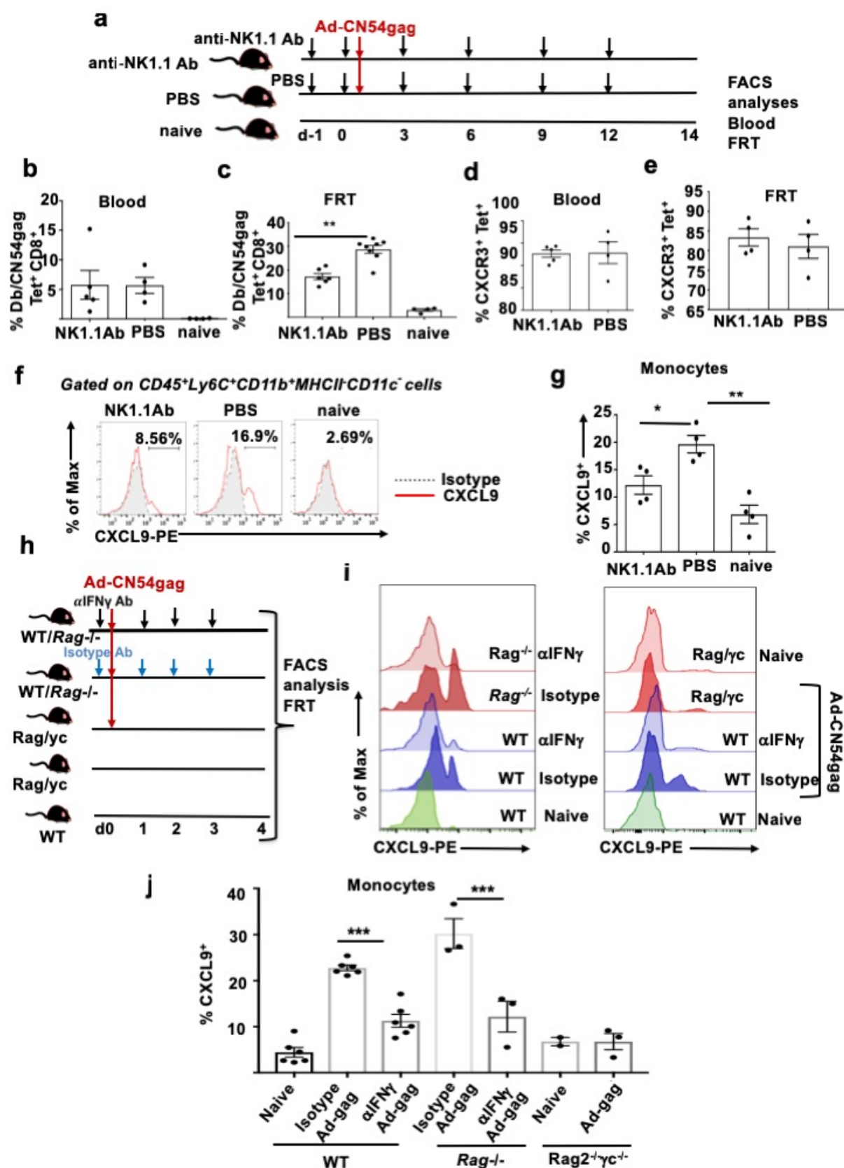
Figure 8. Recruitment of CD8 + T cells to the FRT requires group 1 ILCs and IFN \gamma (a)
