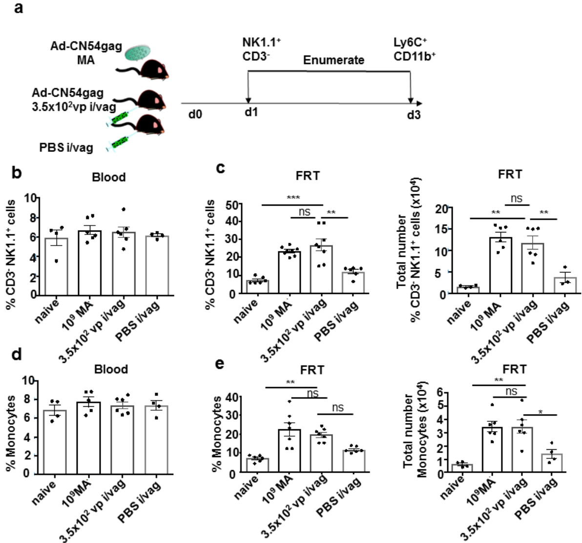
Figure 7. Ad-vector bio-distributed after skin immunisation recruits group 1 ILCs and monocyte into the FRT. (a) Experimental design. Mice were immunised with Ad-CN54 gag by MA delivery to skin (1x10 9 vp) or by injection to the vaginal mucosa (i/vag) with 3.5x10 2 vp (equivalent to the bio-distributed Ad vector dose). Control mice were injected PBS (i/vag.). After 1 day, NK1.1 + CD3 - (ILC1) and after 3 days (monocytes) were enumerated from peripheral blood and FRT tissues. (b) Frequency of Lin - NK1.1 + CD3 - ILC1 in peripheral blood. (c) Frequency (left panel) and absolute number (right panel) of Lin - NK1.1 + CD3 - ILC1 in FRT. (d) Frequency of monocytes in peripheral blood. (e) Frequency (left panel) and absolute number (right panel) of monocytes cells in FRT. Data are from two independent
