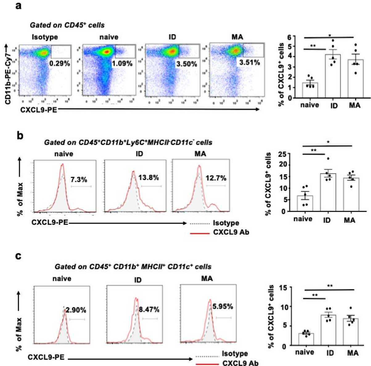
Figure 5. Monocytes infiltrating the FRT express the CXCR3 ligand CXCL9 after skin immunisation. (a) Representative flow cytometry plots and summary bar graph of CXCL9 expressed on CD45 + CD11b + cells isolated from FRT tissue at day 7 after skin immunisation with Ad-CN54 gag via ID injection or MA application or left naive. (b,c) Representative histograms and bar graphs summarise CXCL9 expression among: (b) a gated CD45 + Ly6C + CD11b + MHCII - CD11c - monocyte population and (c) a gated CD45 + Ly6C - CD11b + MHCII + CD11c + dendritic cell population. Data are representative of three independent experiments (n=5 per experimental group). *p<0.05, **p<0.01 by one-way ANOVA, error bars show s.e.m.
