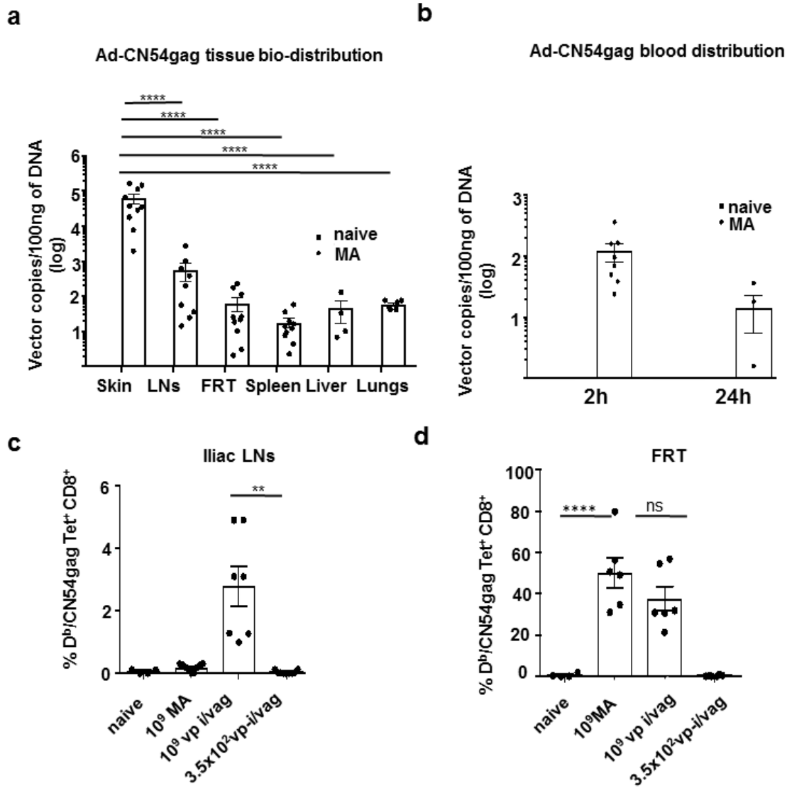
Figure 3. Bio-distributed rAd5 vaccine vector does not prime CD8 + T cells in FRT or iliac LNs. (a) Quantification of Ad vector genomes by qPCR sequestered in indicated organs at 24 h post-MA immunisation with Ad-CN54 gag (1 x 10 9 vp). (b) Ad vector genomes quantified in whole blood at 2 and 24 h post skin (MA) immunisation with Ad-CN54 gag (1 x 10 9 vp) (a,b). Data are from 2 independent experiments (n= 4-10 per group). (c,d) Frequencies D b /CN54 gag tet + CD8 + T cells in FRT tissue and iliac LNs after skin (MA) or intra-vaginal immunisation with Ad-CN54 (1 x 10 9 vp) or with the vector dose (3.5 x 10 2 vp) equivalent to the copy number detected by qPCR in FRT after skin immunisation. Data (n=4-9 per group) are from three independent experiments. P>0.05 (ns), **p<0.01, ***p<0.001 by one-way ANOVA, error bars show s.e.m.
