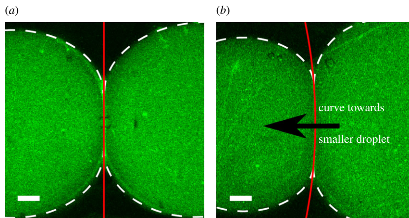
Figure 2. Filtered CLSM image (a) of a volume-symmetric DIB formed from a single lipid type and (b) of a volume-asymmetric DIB (volume ratio of 0.37) that exhibits bilayer interface curvature. Both droplets consist of DPhPC with dilute (0.1% molar fraction) NDB-PC dye formed in hexadecane. The bilayer concavity faces the smaller droplet with higher Laplace pressure. Scale bars, 100 \mu\text{m} .
