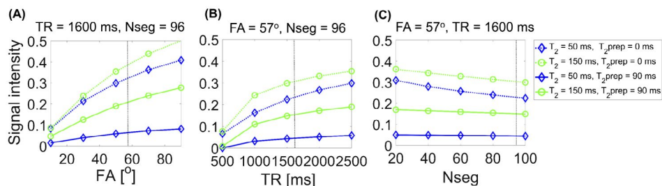
FIGURE 1 Simulated signal intensity as a function of acquisition parameters FA (A), TR (B), and N_{\text{seg}} (C). The signal intensity for each parameter value was obtained from the magnetization response corresponding to T_2 prep duration = 0 ms (dotted lines) or T_2 prep duration = 90 ms (solid lines). The tissues simulated are T_1^{\text{blue}} = 1700 ms, T_2^{\text{blue}} = 50 ms (blue lines), and T_1^{\text{green}} = 1700 ms, T_2^{\text{green}} = 150 ms (green lines)
