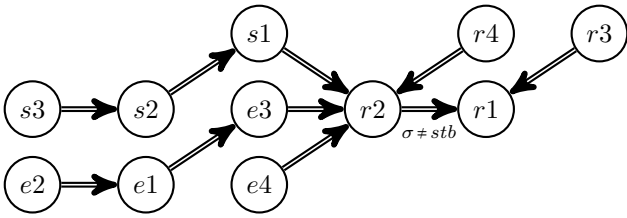
Figure 1: Dependencies
