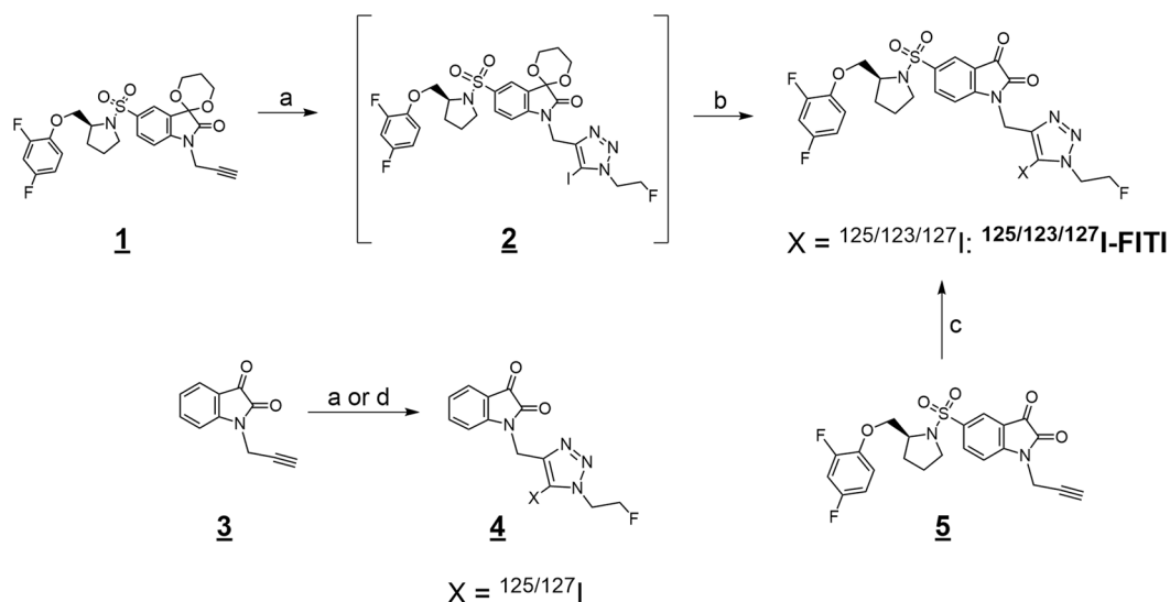
Figure 2. Reaction schemes. Synthesis of [ ^{123}/^{125}/^{127}I ]FITI and the negative control compound 4 . Reaction conditions: (a) 2-fluoroethyl azide, CuI, NEt 3 , N -iodosuccinimide, MeCN, 3 h, r.t.; (b) 4 M HCl, MeCN, reflux, 1 h.; (c) [ ^{125}I ]NaI, bathophenanthroline/CuCl 2 , NEt 3 , 2-fluoroethyl azide, MeCN, 60 min, r.t.; (d) [ ^{125}I ]NaI, bathophenanthroline/CuCl 2 , 2-fluoroethyl azide, MeCN, 60 min, r.t.
