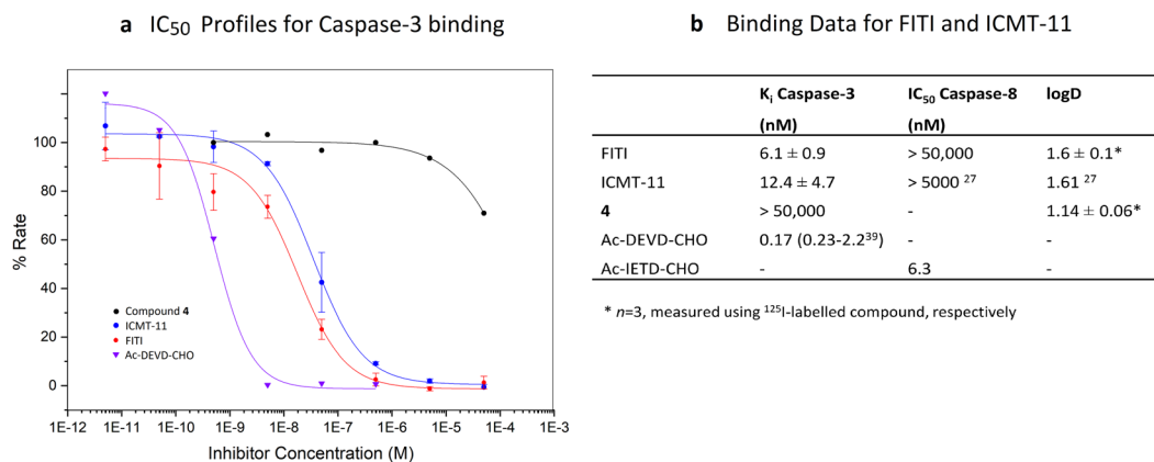
Figure 4. In vitro data. (a) \text{IC}_{50} profiles for caspase-3 binding of FITI, ICMT-11, compound 4, and Ac-DEVD-CHO. Data for compound 4 and Ac-DEVD-CHO are averages of three experiments from one assay plate. Data for FITI and ICMT-11 are averages of three assay plates from three experiments each with standard deviations shown. (b) Table showing caspase-3 and caspase-8 39 binding data for FITI, ICMT-11 and compound 4.
