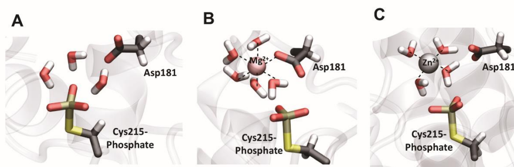
Figure 4. The active site of PTP1B in a representative snapshot at the end of the QM/MM MD simulations. (A) Structure in the absence of metal ions, and (B) Mg^{2+} and (C) Zn^{2+} bound systems. Residues Cys215phosphate, Asp181 and water molecules in the active site or coordinating the metal are shown in licorice representation. C atoms are depicted in black, S atoms in yellow, O atoms in red and H atoms in white. Protein secondary structural elements are shown as white transparent surfaces.
