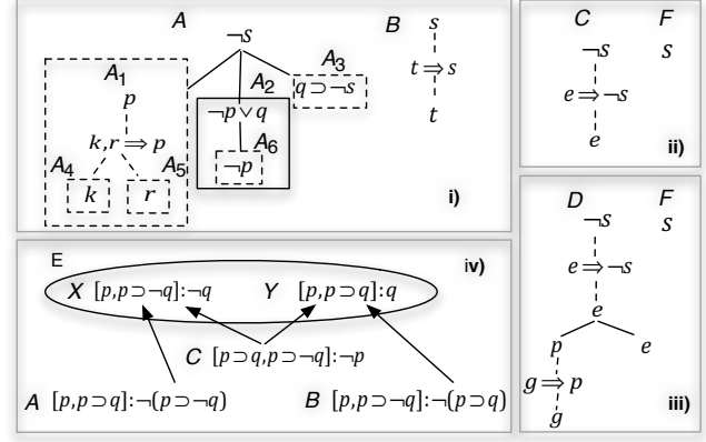
Figure 1: ASPIC + arguments.
