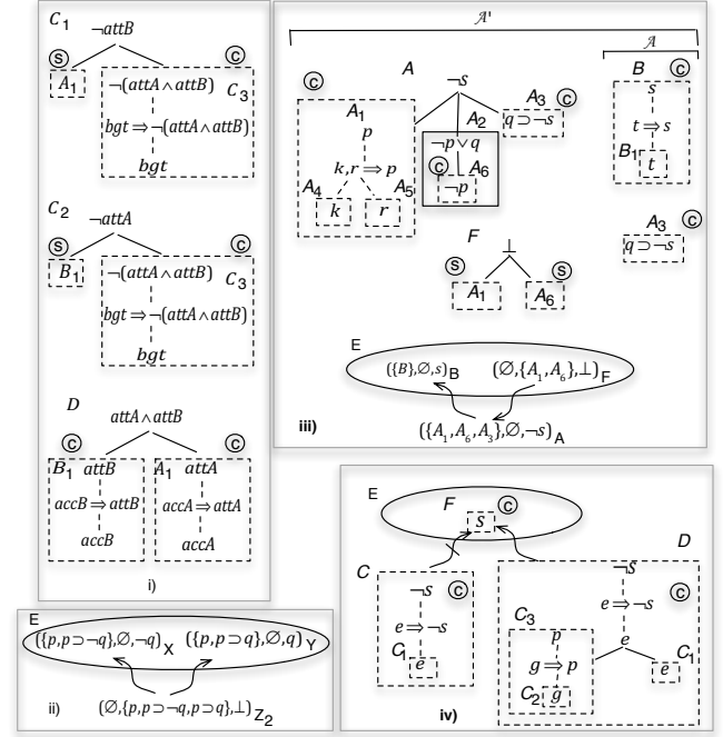
Figure 2: D-ASPIC^+ arguments.
