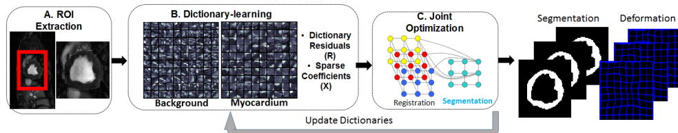
Fig. 1: Algorithm design for joint segmentation and registration. Region of interest extraction (Panel A). Dictionary learning from training images and calculation of residuals (R) and sparse coefficients(X) (Panel B). Multi-resolution deformation grids and exemplary connections with segmentation grid (Panel C)
