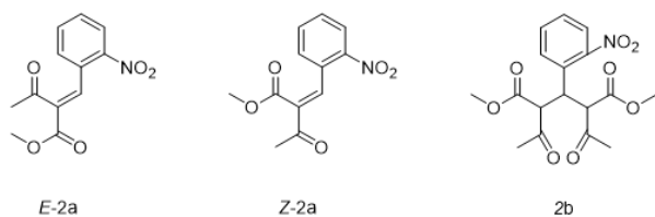
Figure 2. Intermediate reaction species formed in the precursor reaction mixture
