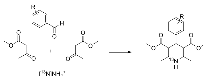
Figure 1. Radiosynthetic reaction scheme for the synthesis of 13 N-labelled 1,4-dihydropyridines
