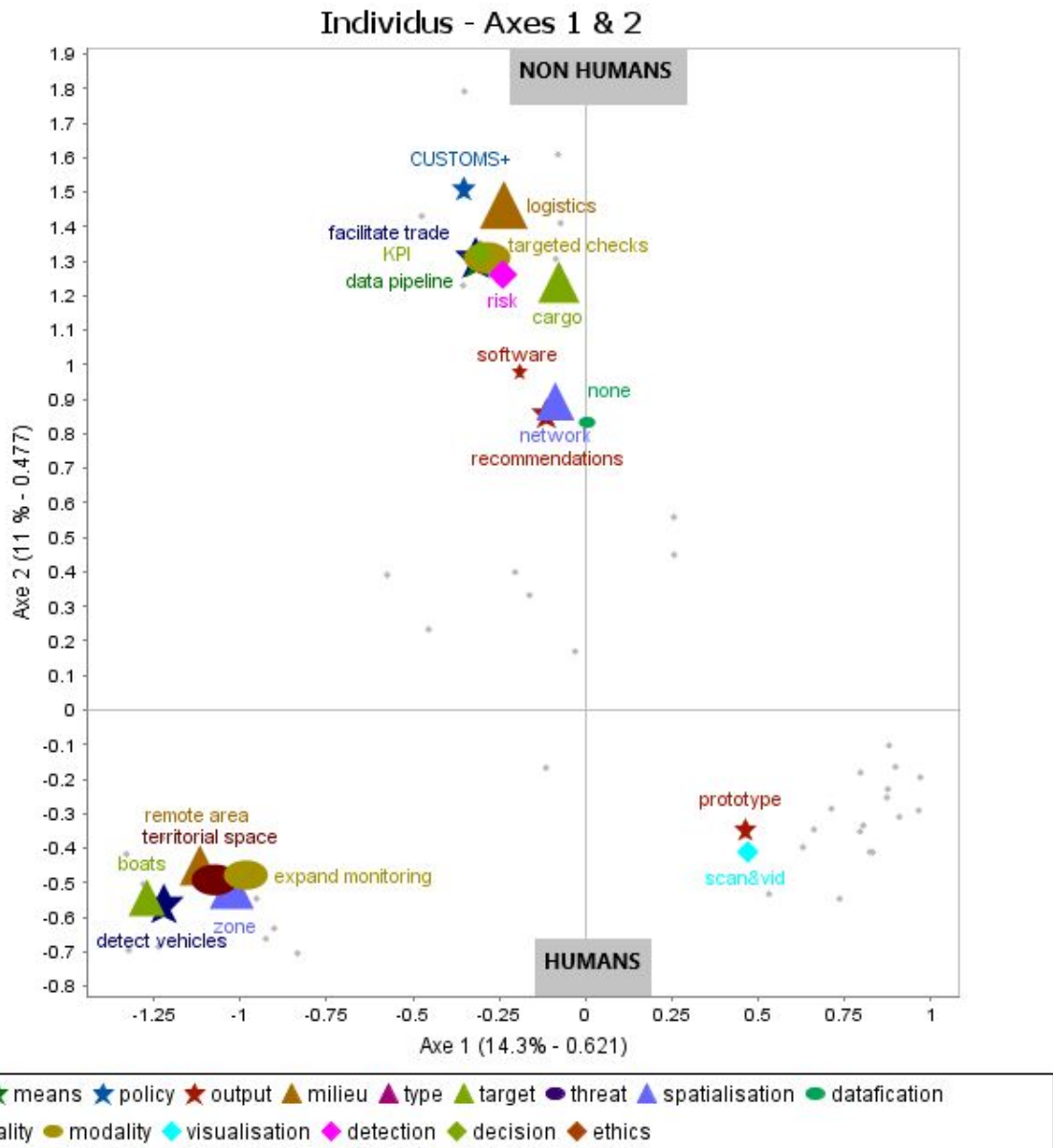
Figure 5. Axis 2
