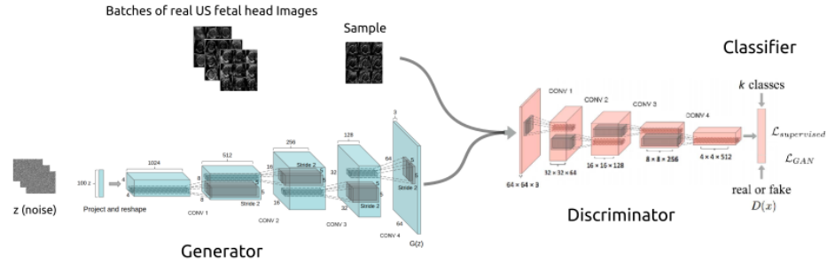
Fig. 1. DCGAN architecture for US imaging. Figure is adapted from the work of Radford et al. 2016 [8].
