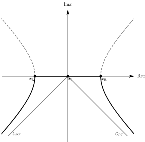
FIG. 2: The deformed contour \mathcal{C}'_{\mathcal{PT}} (heavy solid line) is composed of steepest-descent paths through the stationary points x_L (left half-hyperboloid), x_0 (the real line), and x_R (right half-hyperboloid).
