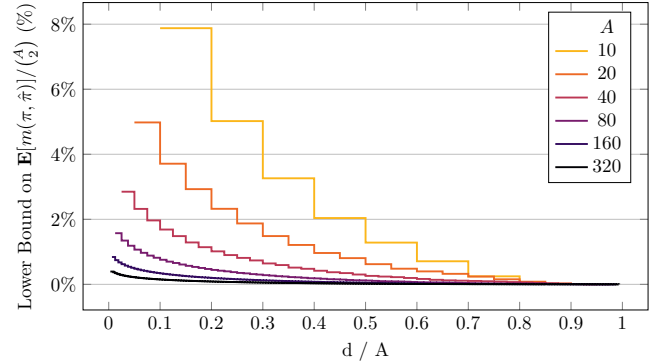
Figure 1: Lower bound on the expected error, as a percentage of the maximum possible error.
