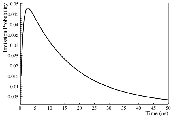
FIG. 1: Parameterised time profile of scintillation light emission for electrons in LAB with 0.6 g/L PPO based on comparisons of ^{214}\text{Bi} background events in data and simulations.
