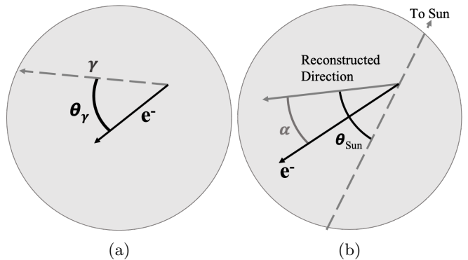
FIG. 2: Definitions of angles referenced in this paper: \theta_\gamma is the angle between the electron’s travel direction and the photon direction; \alpha is the angle between the true and reconstructed direction of the electron; and \theta_{\text{Sun}} is the angle between the reconstructed event direction and the solar direction (assumed true direction of the neutrino).
