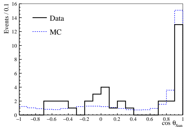
FIG. 6: Results of direction reconstruction for measured (solid) and simulated (dashed) ^8\text{B} solar neutrinos, where simulation sampled from a nominal ^8\text{B} energy spectrum.
