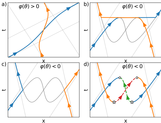
FIG. 1. Trajectories of two particles during scattering for a) \varphi(\theta) > 0 and b), c), d) \varphi(\theta) < 0 . The thin dashed lines are the asymptotic trajectories. We show three interpretations of the multivalued solutions for \varphi(\theta) < 0 : b) Particles jump instantaneously. c) Particles are relabelled during collisions. d) Spontaneous creation of a particle-antiparticle pairs: starting from the bottom, at a certain time (marked by a star) the blue and orange particles are close enough to allow for two pair creations (there are 3 solutions: two blue-orange (outer), one red-green (inner)). Later one particle of each pair (the red and green) each annihilates one of the original particles (marked by a circle), leaving the new blue and orange particles as outgoing.. We used \psi(x, \theta) = \frac{x}{\sqrt{x^2 + \alpha^2}} 2 \arctan \frac{\theta}{c} , with c = 0.5, \alpha = 0.4 for a) and c = -1, \alpha = 1 for b), c), d).
