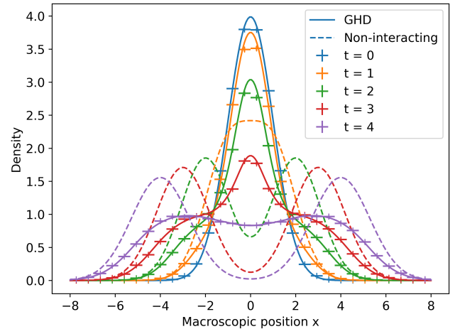
FIG. 2. Evolution of the microscopic particle density (data points) and that from the GHD solution (solid lines) for different times. The initial state is \rho_p(\theta, x, 0) = \frac{25}{2\pi} e^{-x^2/2} \left( e^{-25(\theta-1)^2/2} + e^{-25(\theta+1)^2/2} \right) . We use \psi(x, \theta) = \frac{x}{2\sqrt{x^2 + \alpha^2}} \phi(\theta) , where \alpha = 0.1 and \phi(\theta) = 2 \arctan \frac{\theta}{c} . The microscopic results were averaged over 100 samples, each starting from a randomly generated initial state ( L = 300 , each sample contains N \approx 3000 particles). The error bars indicate the standard deviation and the bin size used for computing the density of particles. We also give the density for non-interacting particles (dashed lines) for comparison.
