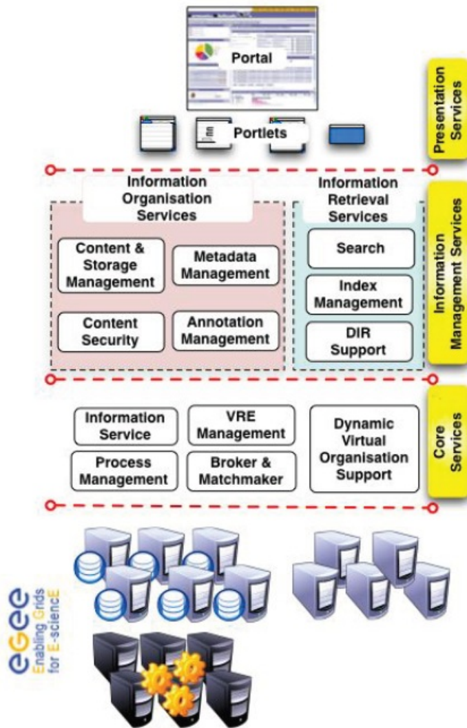
Figure 1. gCube Architecture
