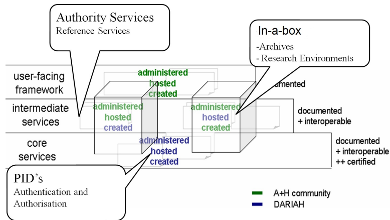
Figure 1. DARIAH architecture
