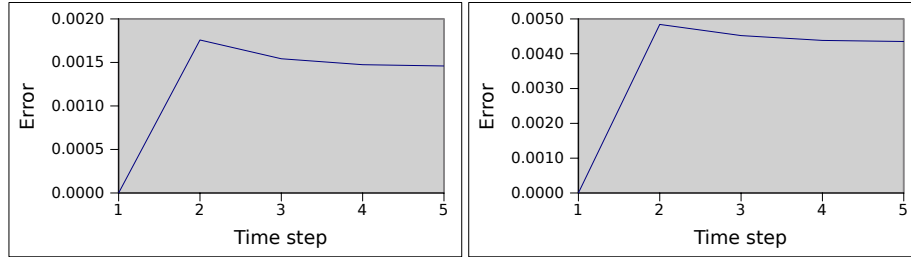
Figure 4: Errors between compositional and non-compositional calculation of transient probabilities for global state HHH (left) and III (right)
