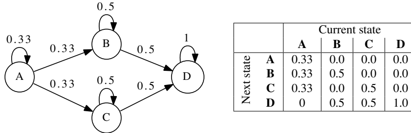
Figure 1: Graph representation and adjacency matrix of a simple agent DTMC
