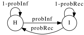
Figure 3: DTMC representation of an agent in the disease transmission simulation
