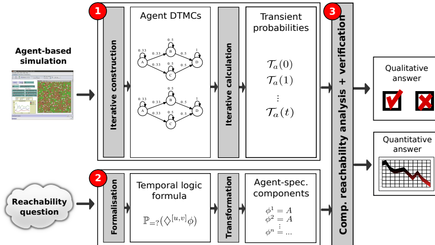
Figure 2: Schematic overview of the verification approach
