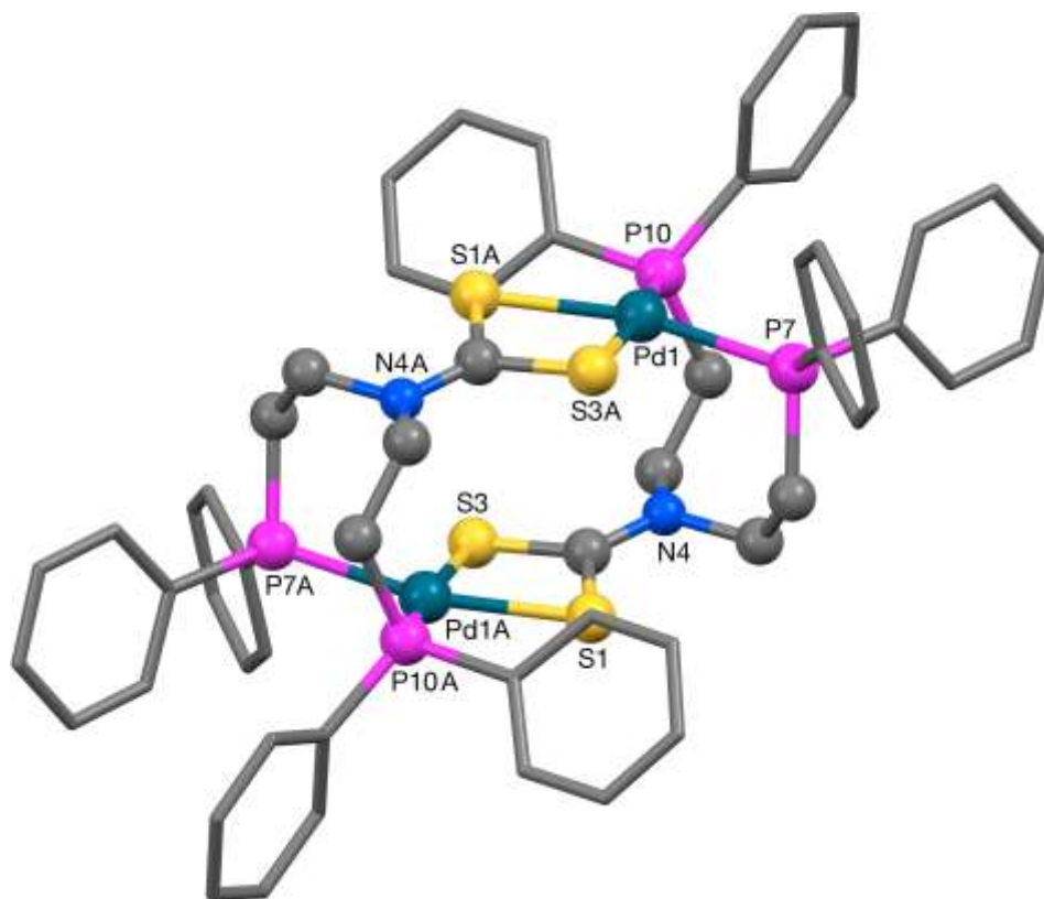
Figure 3. The molecular structure of [\text{Pd}\{\text{S}_2\text{CN}(\text{CH}_2\text{CH}_2\text{PPh}_2)_2\}]_2(\text{Cl})_2 ( 9 ) with the counteranions omitted for clarity. Selected bond lengths ( \text{\AA} ) and angles ( ^\circ ): \text{Pd}(1)\text{--P}(10) = 2.2702(10) , \text{Pd}(1)\text{--P}(7) = 2.2978(11) , \text{Pd}(1)\text{--S}(1\text{A}) = 2.3371(10) , \text{Pd}(1)\text{--S}(3\text{A}) = 2.3438(10) , \text{S}(1)\text{--C}(2) = 1.714(4) , \text{S}(1)\text{--Pd}(1\text{A}) = 2.3372(10) , \text{C}(2)\text{--N}(4) = 1.327(5) , \text{C}(2)\text{--S}(3) = 1.725(4) , \text{S}(3)\text{--Pd}(1\text{A}) = 2.3438(10) , \text{P}(10)\text{--Pd}(1)\text{--P}(7) = 97.21(4) , \text{P}(10)\text{--Pd}(1)\text{--S}(1\text{A}) = 95.97(4) , \text{P}(7)\text{--Pd}(1)\text{--S}(3\text{A}) = 91.02(4) , \text{S}(1\text{A})\text{--Pd}(1)\text{--S}(3\text{A}) = 74.99(3) , \text{S}(1)\text{--C}(2)\text{--S}(3) = 111.9(2) .
