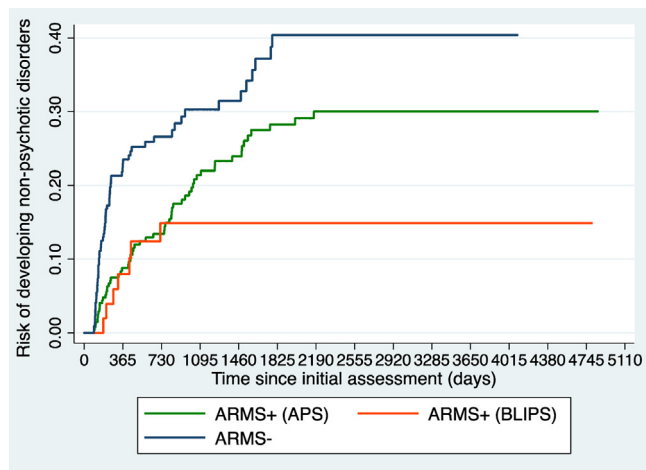
Fig. 3. Cumulative incidence (Kaplan–Meier failure function) for the long-term risk of development of non-psychotic disorders in At Risk Mental State (ARMS)+ (APS) ( n = 299 ), ARMS+ (BLIPS) ( n = 62 ) and ARMS– ( n = 228 ) subjects.
