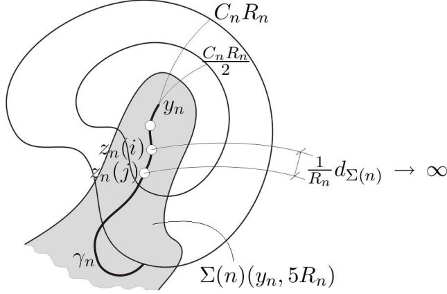
Figure 2: d_{\Sigma(n)} denotes the intrinsic distance in \Sigma(n) .
