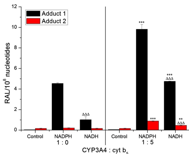
Fig. 7 DNA adduct formation (RAL, relative adduct labelling) by ellipticine activated with human CYP3A4 in the presence of either NADPH or NADH and the effect of cytochrome b 5 (cyt b 5 ) (at a molar ratio of CYP3A4:cytochrome b 5 of 1:5) on this reaction. Values represent mean total RAL (relative adduct labeling) \pm SD ( n = 3 ; analyses of three independent in vitro incubations). \Delta\Delta\Delta P < 0.001 (Student's t test), levels of ellipticine-derived DNA adducts significantly different from incubations with NADPH as a cofactor; ***P < 0.001 (Student's t test), levels of ellipticine-derived DNA adducts significantly different from incubations without cytochrome b 5 . Control—incubations without added cofactors
