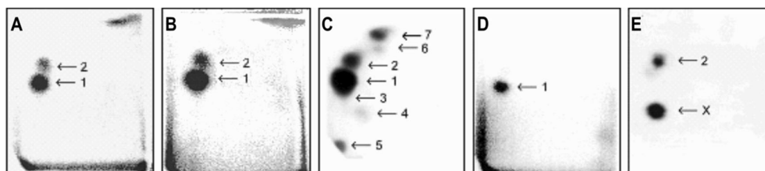
Fig. 5 Autoradiographic profile of ^{32}\text{P} -labeled DNA adducts generated in calf thymus DNA by ellipticine after its activation with CYP3A4 in the presence of NADPH without (a) and with cytochrome b_5 (CYP3A4:cytochrome b_5 of 1:5) (b): of ^{32}\text{P} -labeled digests of DNA from the liver of a male rat treated with 40 mg ellipticine per kg
