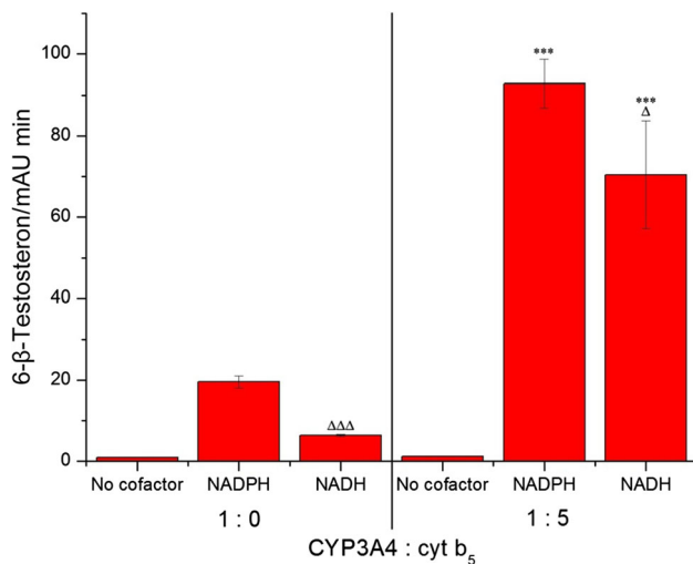
Fig. 3 Testosterone 6- \beta -hydroxylation catalyzed by CYP3A4-Supersomes TM with and without cytochrome b_5 (at a molar ratio of CYP3A4:cytochrome b_5 of 1:5) in the presence of NADPH or NADH. Data shown are mean peak areas relative to the internal standard phenacetin \pm SD ( n = 3 ; analyses of three independent in vitro incubations). ND not detected. ΔΔΔ P < 0.001 , Δ P < 0.05 (Student's t test), significantly different from incubations in the presence of NADPH as a cofactor; *** P < 0.001 (Student's t test), significantly different from incubations without cytochrome b_5
