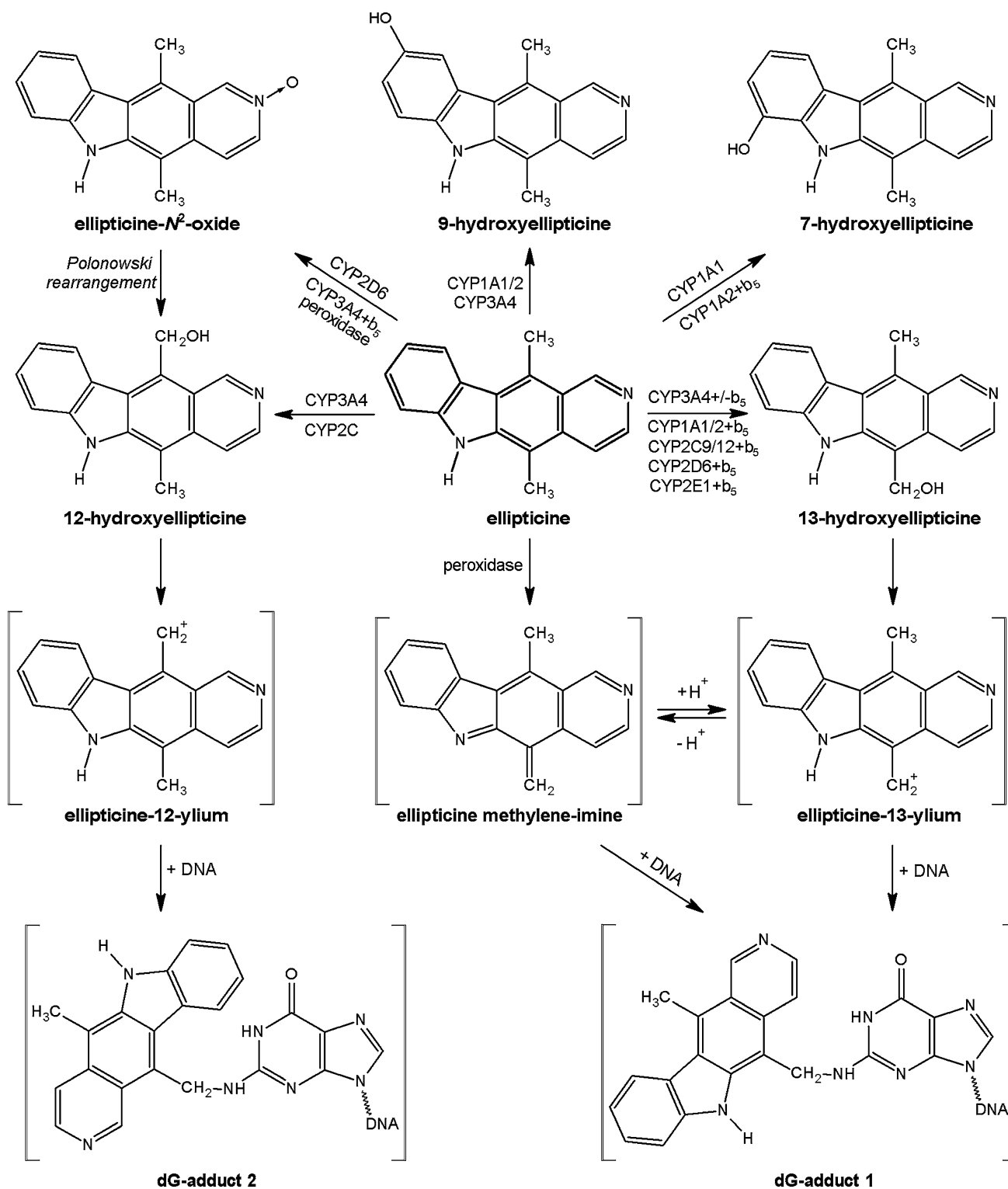
Fig. 1 Scheme of ellipticine metabolism by CYPs and peroxidases showing the identified metabolites and those proposed to form DNA adducts. The compounds shown in brackets were not detected under
