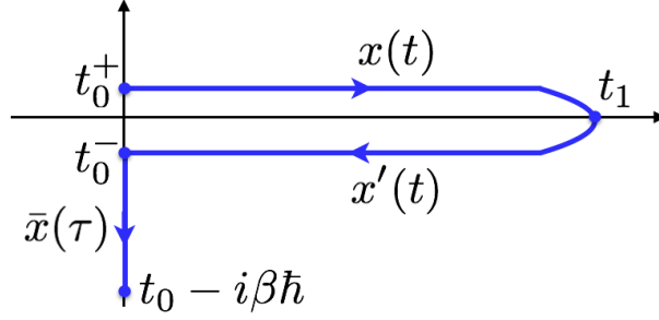
Figure 1: Konstantinov-Perel's contour \gamma . On the horizontal upper (forward) track of the contour \gamma the coupling part of the Hamiltonian depends explicitly on the fixed nuclear trajectory x(t) , the horizontal lower (backward) track - on the fixed nuclear trajectory x'(t) , while the vertical track - on the fixed nuclear trajectory \bar{x}(\tau) corresponding to Euclidean evolution.
